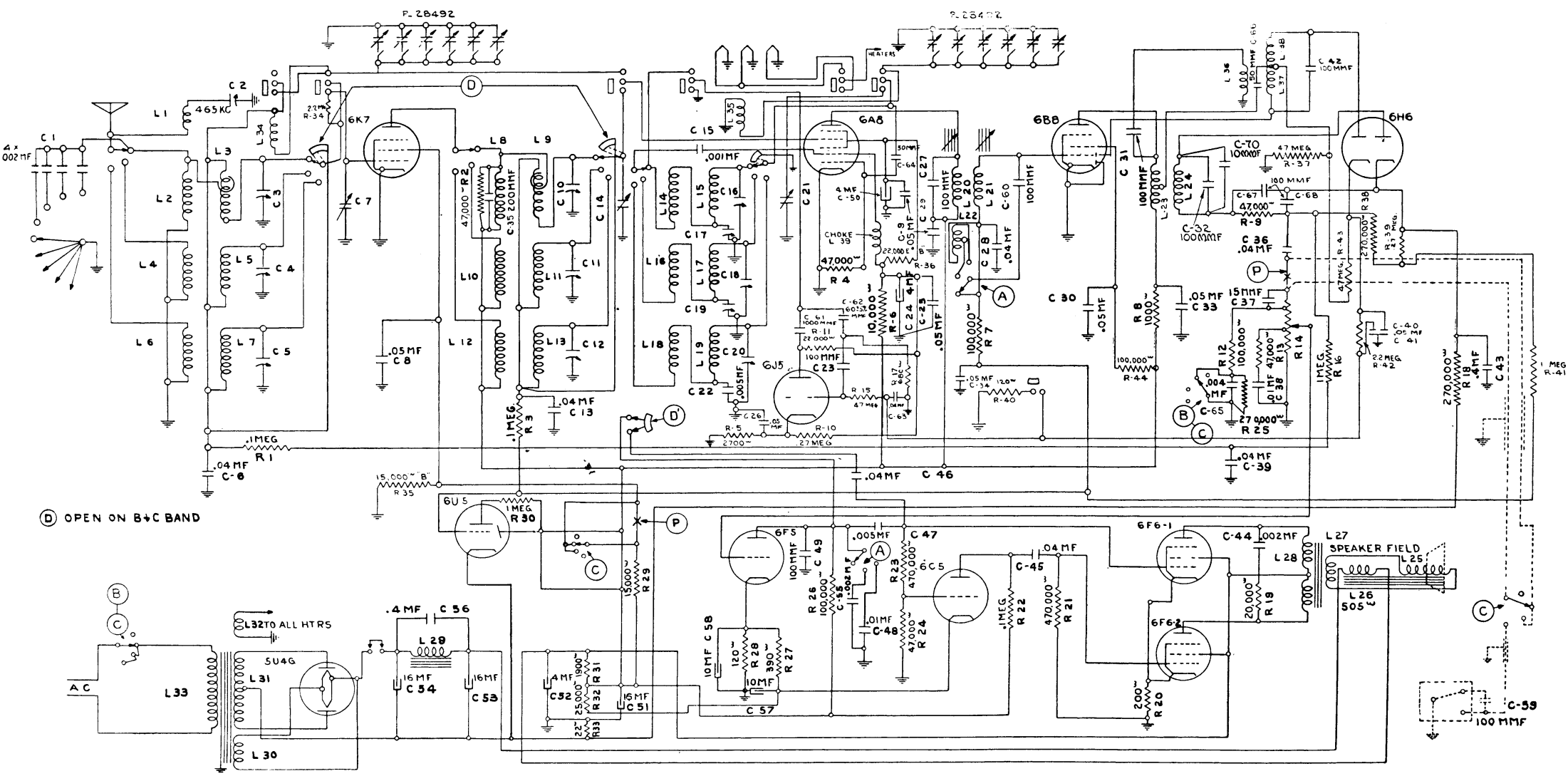
Fig. 3. Schematic Circuit of Receiver.
